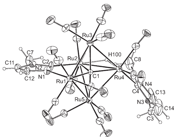
Figure 2. Molecular structure of the carbide cluster 4 (ellipsoids set at 30% probability). Selected bond lengths [Å]: Ru1–N1 2.12(2), Ru1–C1 2.09(2), Ru2–C1 2.07(2), Ru2–C2 2.07(2), Ru3–C1 1.99(2), Ru4–C1 2.07(2), Ru4–C4 2.15(3), Ru5–C1 1.97(2).
