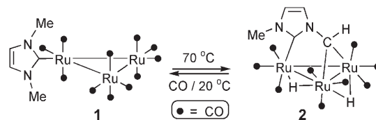
Scheme 1. Reversible activation of two C–H bonds of \text{Me}_2\text{Im} .
